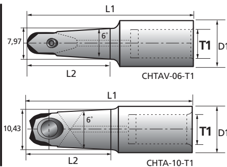
CHTA-10-T1
