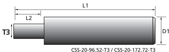
CSS-20-96.52-T3 / CSS-20-172.72-T3
